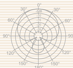
Polar Pattern
