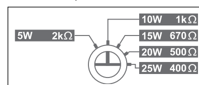
Power Tap Selection UHC-25XT
