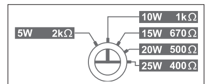
Power Tap Selection UHC-25XT
